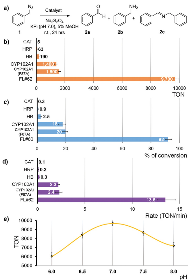
Figure 1. a) Catalytic activity of various hemoproteins in the oxidative deamination of benzyl azide (1) to benzaldehyde (2a). b, c) Reactions (400 \mu\text{L} ) were conducted under anaerobic conditions with 10 mM \text{BnN}_3 , 10 mM \text{Na}_2\text{S}_2\text{O}_4 , and 1 \mu\text{M} protein for 24 h at room temperature. TON = nmol aldehyde/nmol catalyst. Product yield is based on conversion of 1 into 2a, as determined by GC. d) Reaction rates as determined over the first 10 min of the reaction. e) TON versus pH plot for FL#62 reaction.
